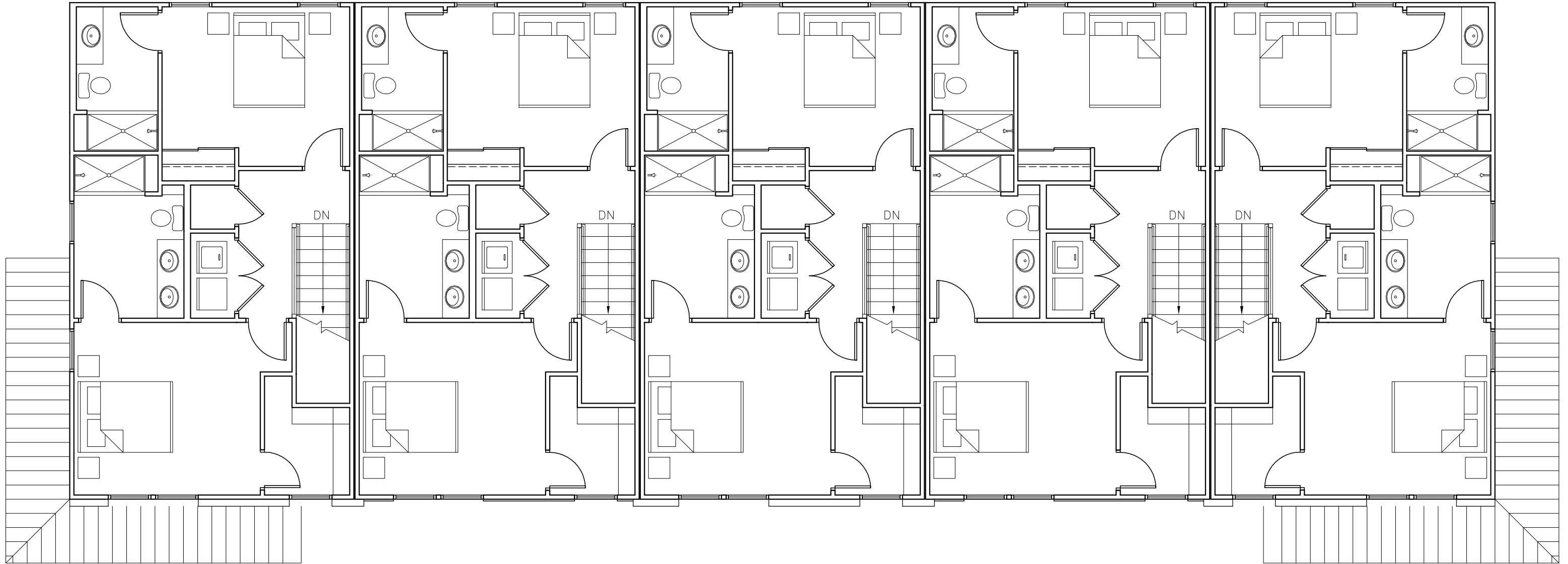
1 THIRD FLOOR 1/4" = 1'-0" N
