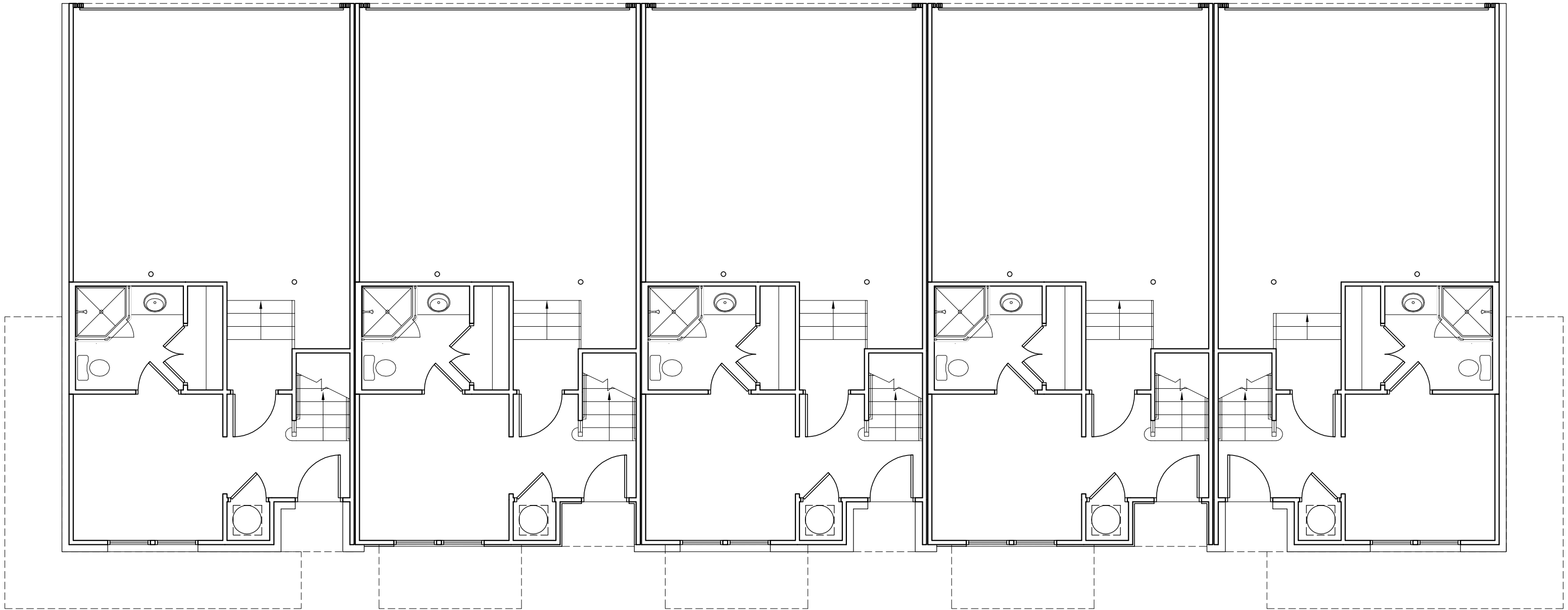
1 FIRST FLOOR 1/4" = 1'-0" N
